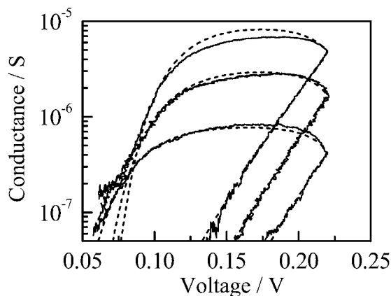
FIGURE 10 Plots of \log G against V for di-alm at pH 3.5 shown in Fig. 7. Sweep rates of voltage (mV/s) were: (top) 0.88, (middle) 2.64, and (bottom) 8.8. The dotted curves indicate best-fit curves calculated using Eq. 6.
